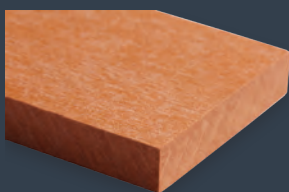
323 - Magma
