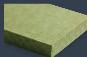
626 - Emerald
